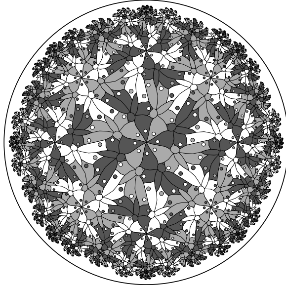
Figure 12: A hyperbolic pattern having 3-color symmetry, based on the \{8, 3\} tessellation and using the butterfly motif of Notebook Drawing Number 70.
