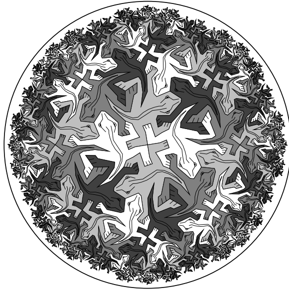
Figure 10: A hyperbolic pattern having 4-color symmetry, based on the \{8,3\} tessellation and using the lizard motif of Notebook Drawing Number 25.
