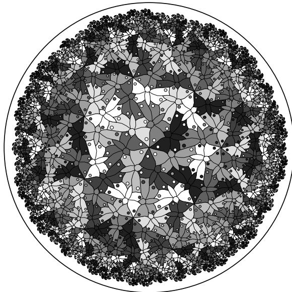
Figure 11: A hyperbolic pattern having 8-color symmetry, based on the \{7,3\} tessellation and using the butterfly motif of Notebook Drawing Number 70.
