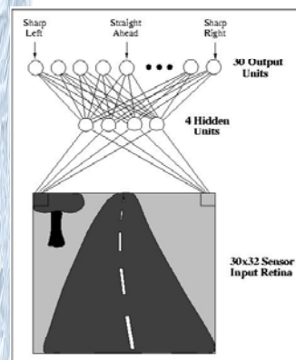
ALVINN [Pomerleau] drives 70 MPH on highways
