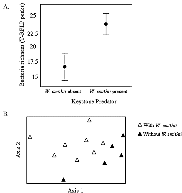
Fig. 6. A. Bacterial richness correlates with presence of the keystone predator (d.f. = 12; F = 7.713 ; P = 0.018 ). Bacterial richness was estimated by the number of T-RFLP peaks measured and the presence of the mosquito larvae was determined by examining the pitcher fluid ( n = 13 ; 8 with mosquito; 5 without). Error bars indicate standard error of the means.
