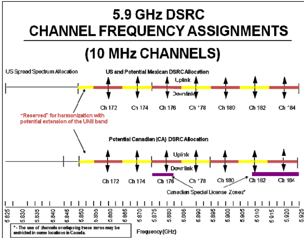
Figure 2.3 - DSRC Channel Frequency Assignments [16]
