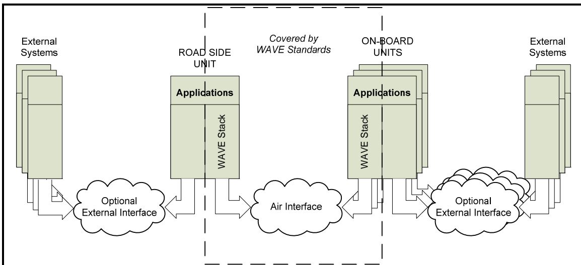
Figure 2.4 - Wave System Components [17]
