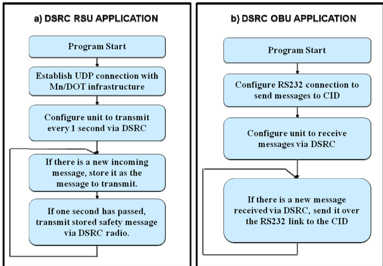
Figure 5.1 - DSRC Unit Application Program Flow: a) RSU, and b) OBU
