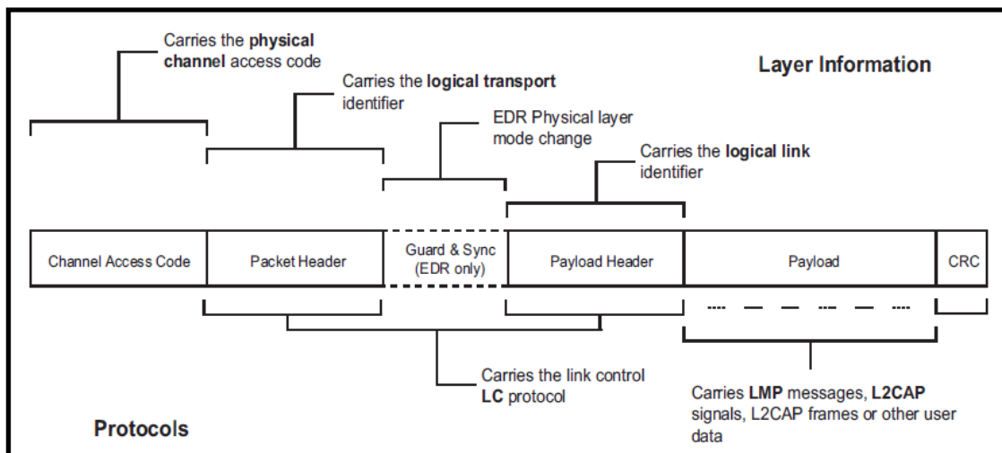
Figure 2.2 - Bluetooth Packet Structure [10]
