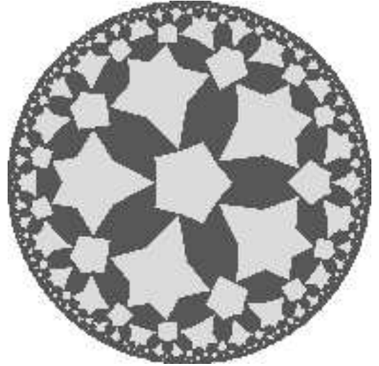
Fig. 5.7. Figure 14
