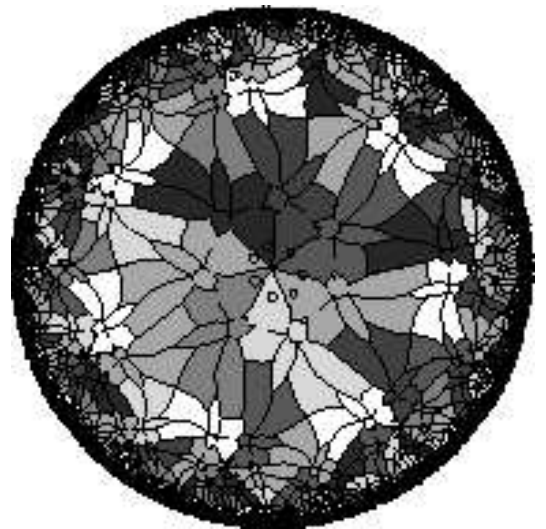
Fig. 5.9. Pattern 70 \{7,4\}
