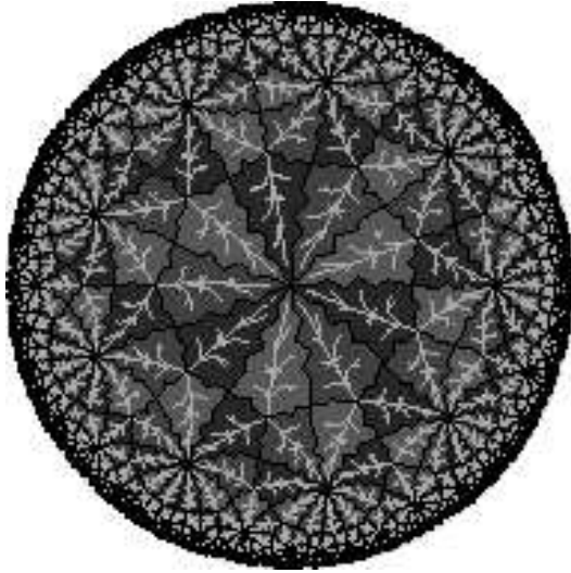
Fig. 5.6. Leaf \{9,3\}
