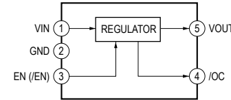
IC406 BD2220G-TR
