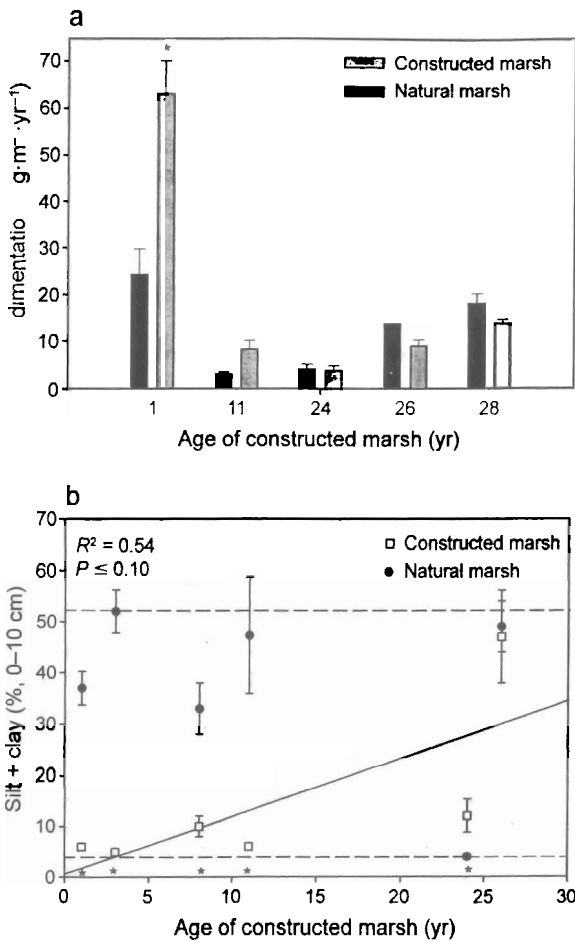
FIG. 7. (a) Sediment deposition and (b) soil silt plus clay (0–10 cm depth) along a chronosequence of constructed salt marshes and natural reference marshes. Asterisks (*) indicate that the constructed and paired reference marshes are significantly different ( P \leq 0.05 ) according to Student's t test. Dashed lines in (b) represent the range of values measured in the natural marshes. The 13-yr-old constructed marsh was excluded from the analysis because of its terrestrial origin (submerged upland) and, hence, high initial clay content.
