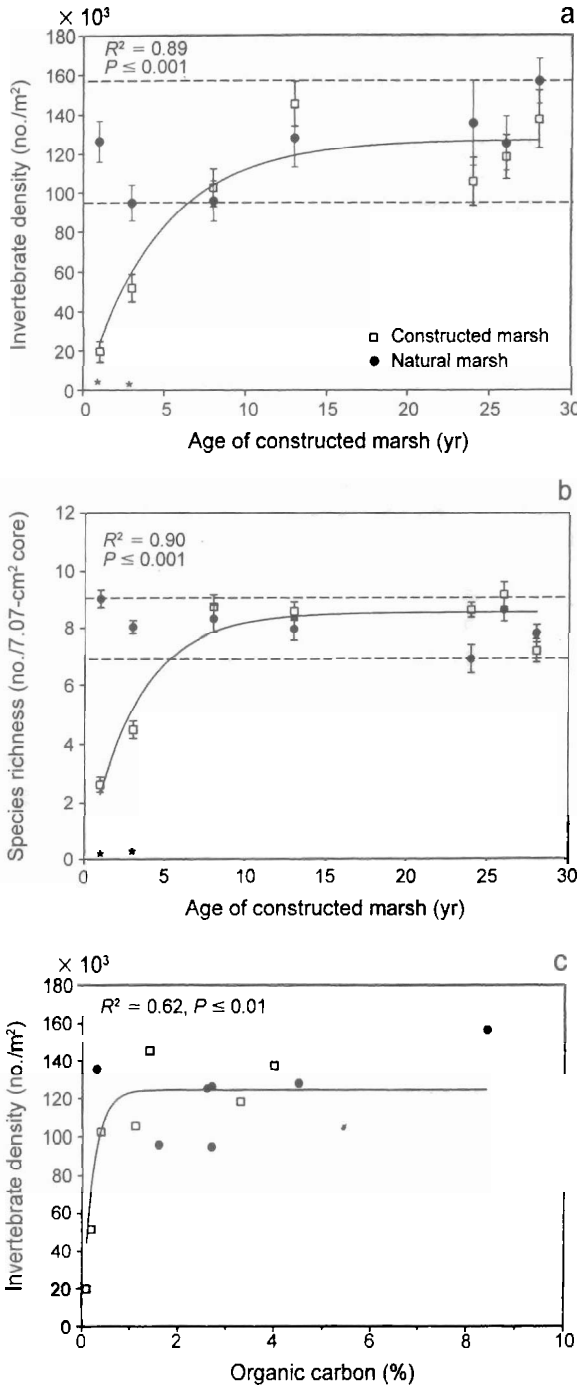
FIG. 6. (a) Density (in thousands per m 2 ) and (b) taxa richness (number of taxa per 7.07-cm 2 core) of benthic invertebrates along a chronosequence of constructed salt marshes and natural reference marshes. Asterisks (*) indicate that the constructed and paired reference marshes are significantly different ( P \leq 0.05 ) according to Student's t test. Dashed lines represent the range of values measured in the natural marshes. (c) Regression of benthic invertebrate density vs. percent soil organic C (0–10 cm depth) of constructed and natural marshes.
