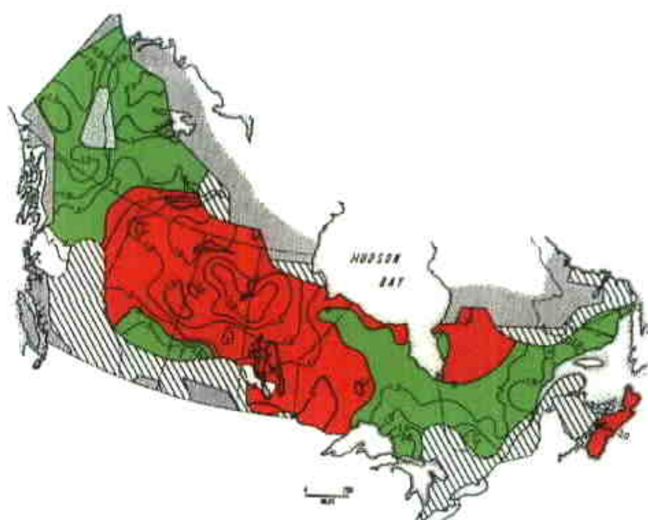
Figure 10. Synchrony in snowshoe hare cycles across Canada, 1931–1948, as measured by questionnaires (Chitty 1948, 1950). The average peak phase across Canada was scaled as 0.0, and the contour lines indicate peaks occurring earlier than average (red, negative contours) or later than average (green, positive contours). During this period, hare peaks were reached earliest in the central boreal region of northern Saskatchewan and Manitoba (Smith 1983).
