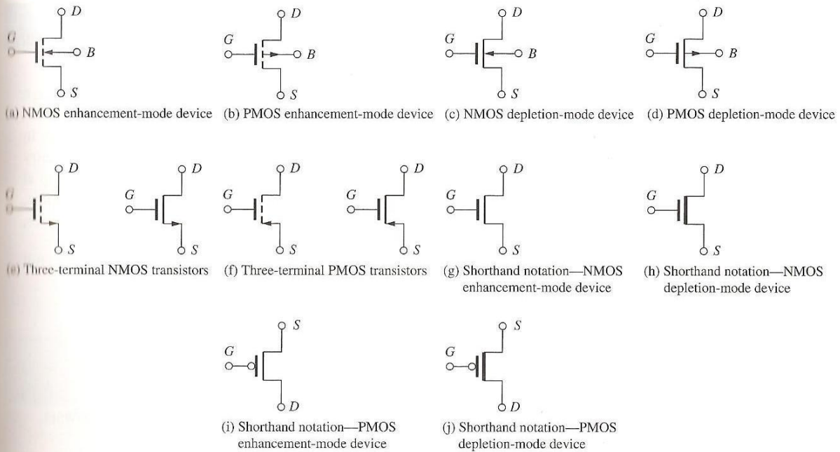
Figure 4.15 (a)–(f) IEEE Standard MOS transistor circuit symbols. (g)–(j) Other commonly used symbols.
