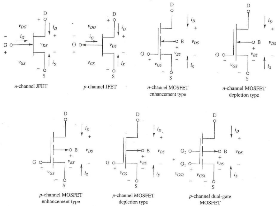
FET circuit symbol summary.
